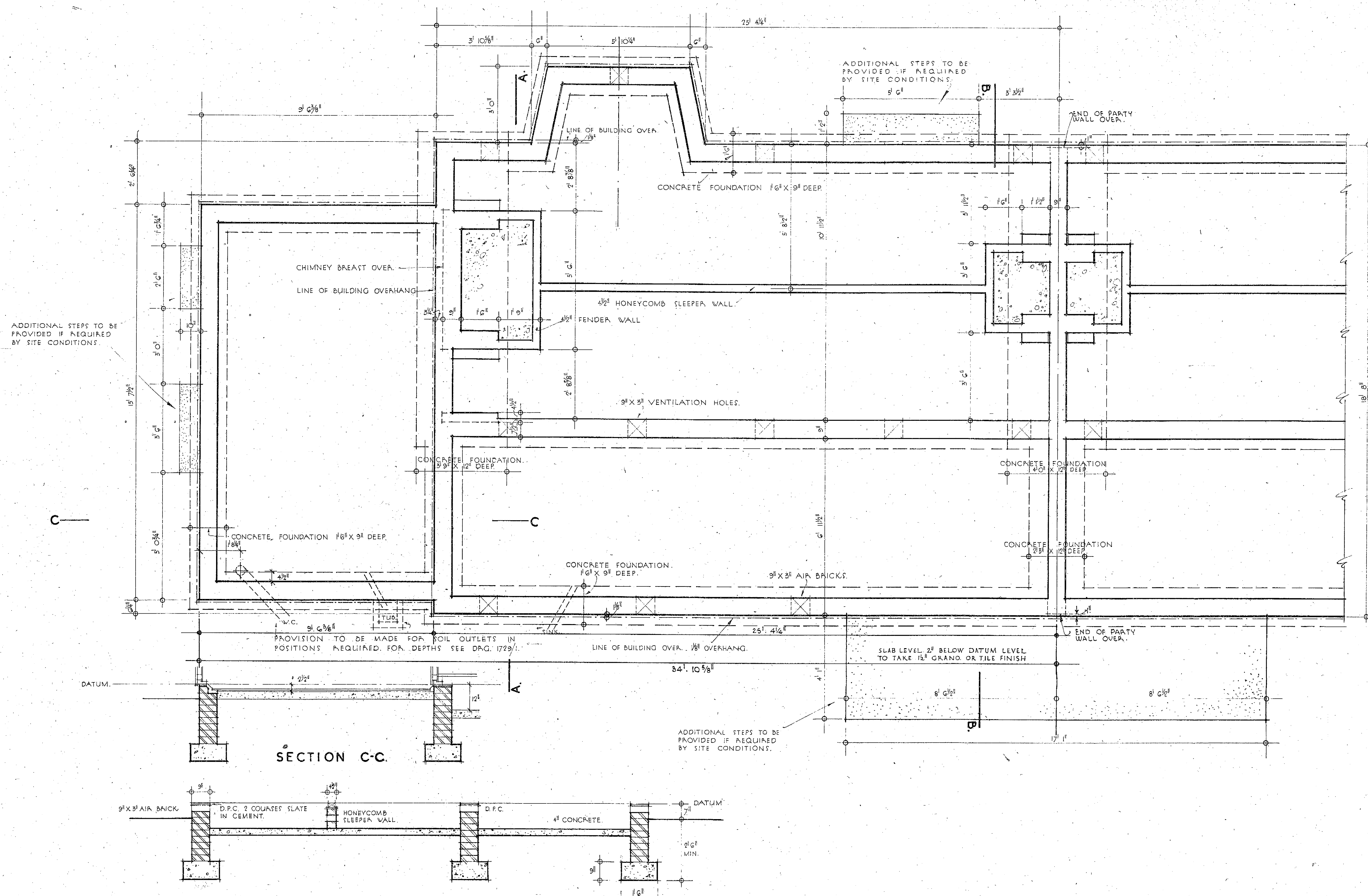
DEPTHS & WIDTHS OF FOUNDATIONS TO BE VARIED TO SUIT SITE CONDITIONS
