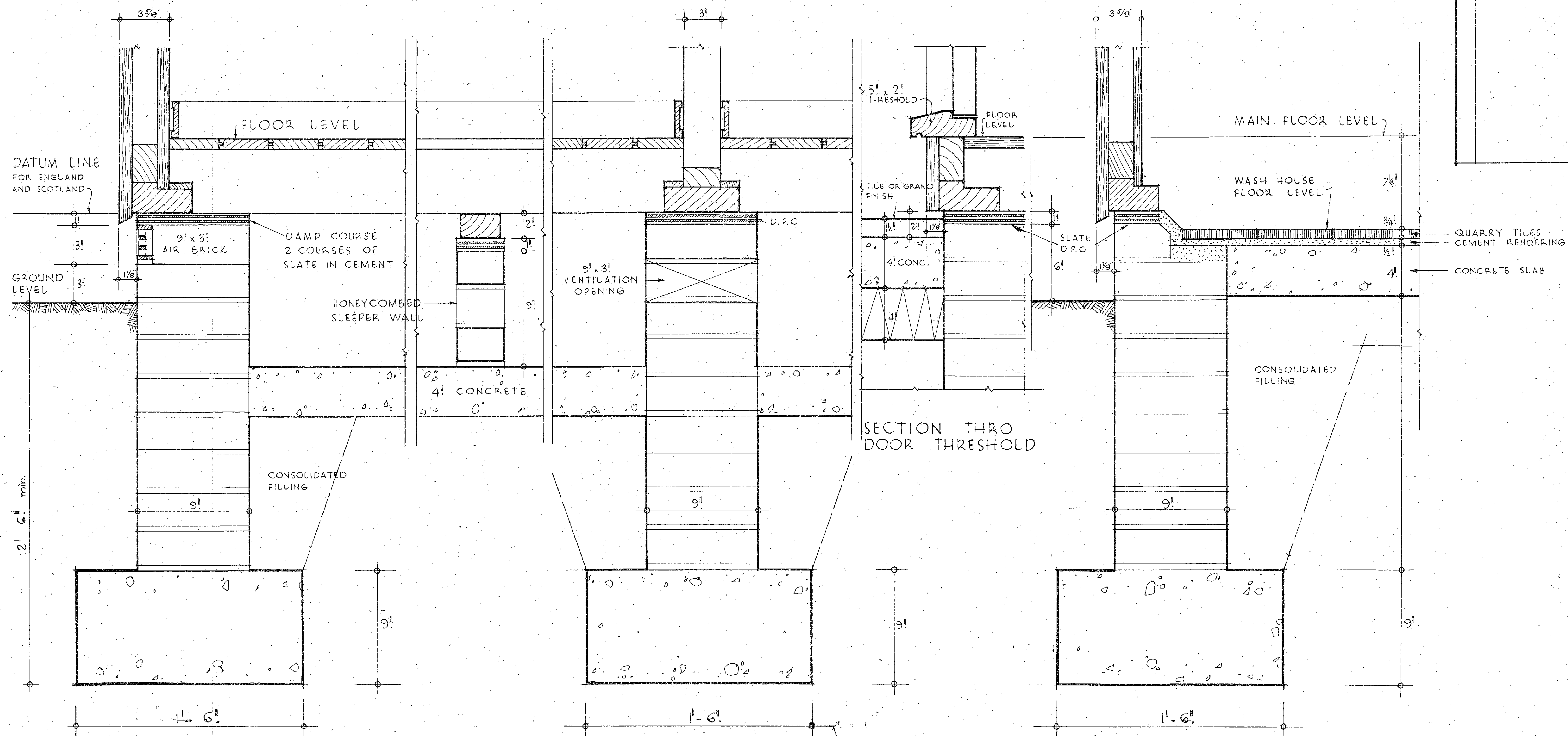
TYPICAL EXTERNAL FOUNDATION
