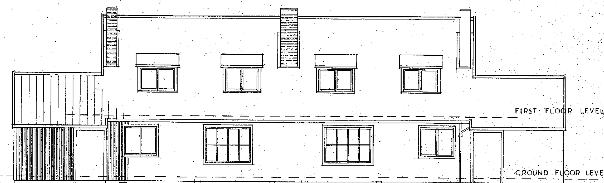
BACK ELEVATION
